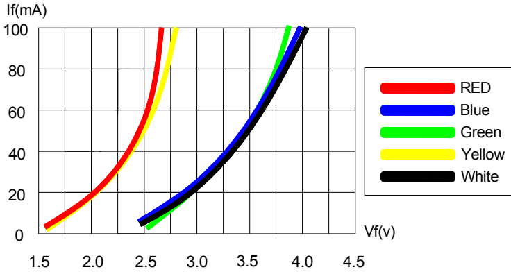
Fig.1 Forward Current vs Forward Voltage)
