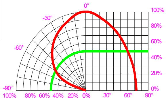
Fig.6 Relative Luminous Intensity vs viewing angle
