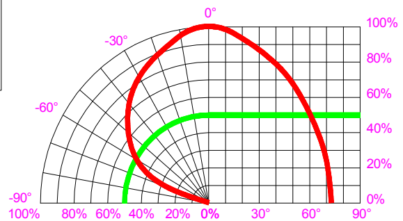
Fig.6 Relative Luminous Intensity vs viewing angle
